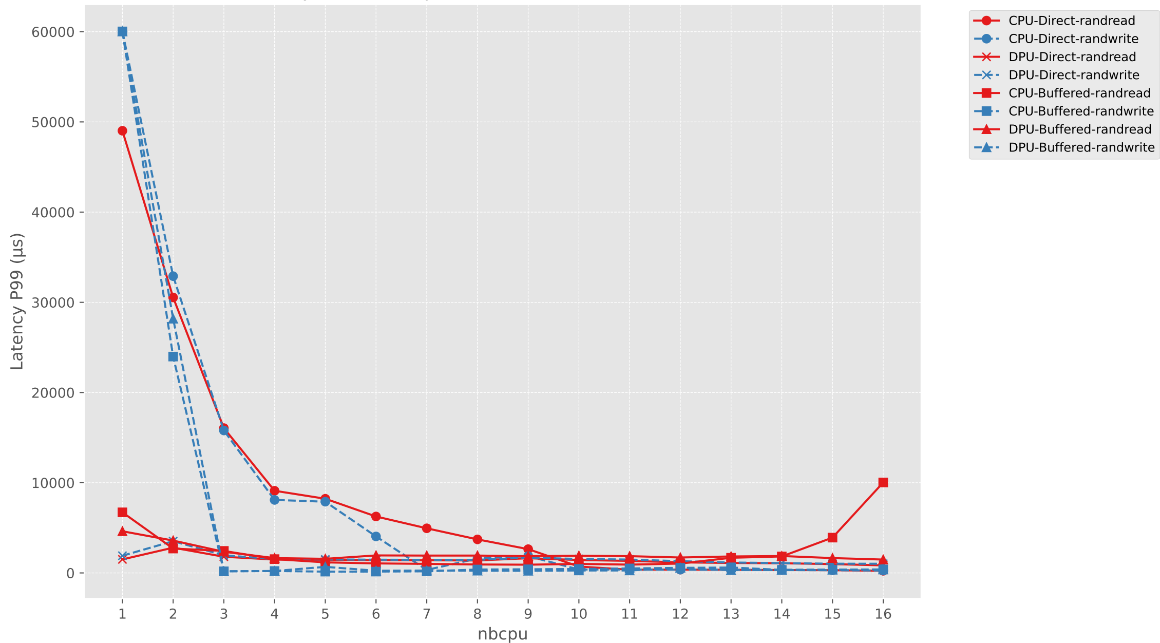
Latency P99 vs nbcpu (CPU vs DPU, Direct vs Buffered)
